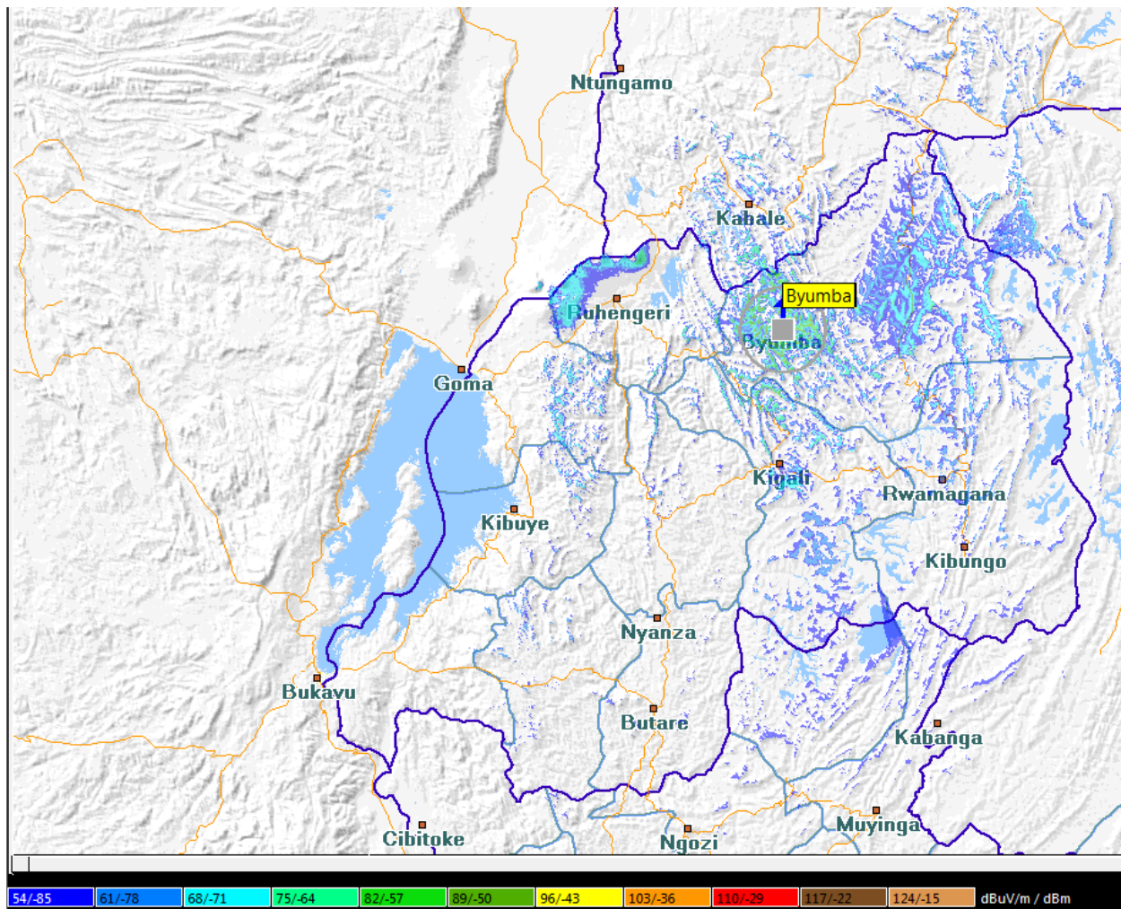
Image 12: Approximate Radio coverage for Ishingiro Radio
