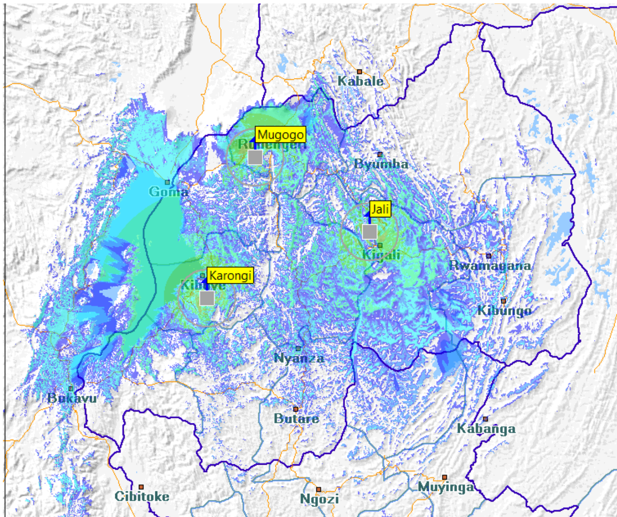
Image 5: Approximate coverage of Energy FM Radio
