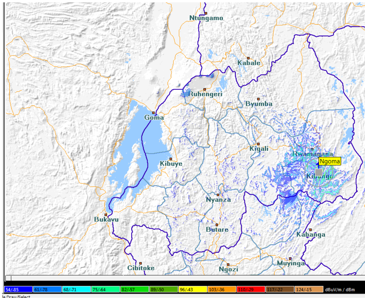
Image 13: Approximate Radio coverage for Izuba radio
