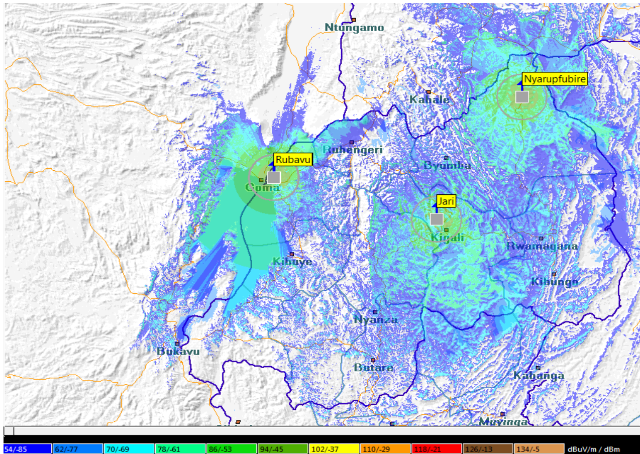
Image 5: Approximate coverage of Radio10 FM
