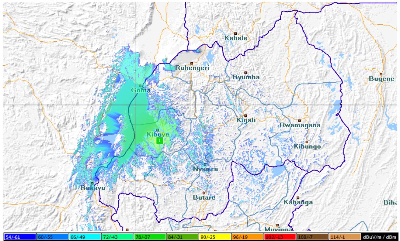
Image 10: Approximate coverage of Isangano radio at Karongi site
