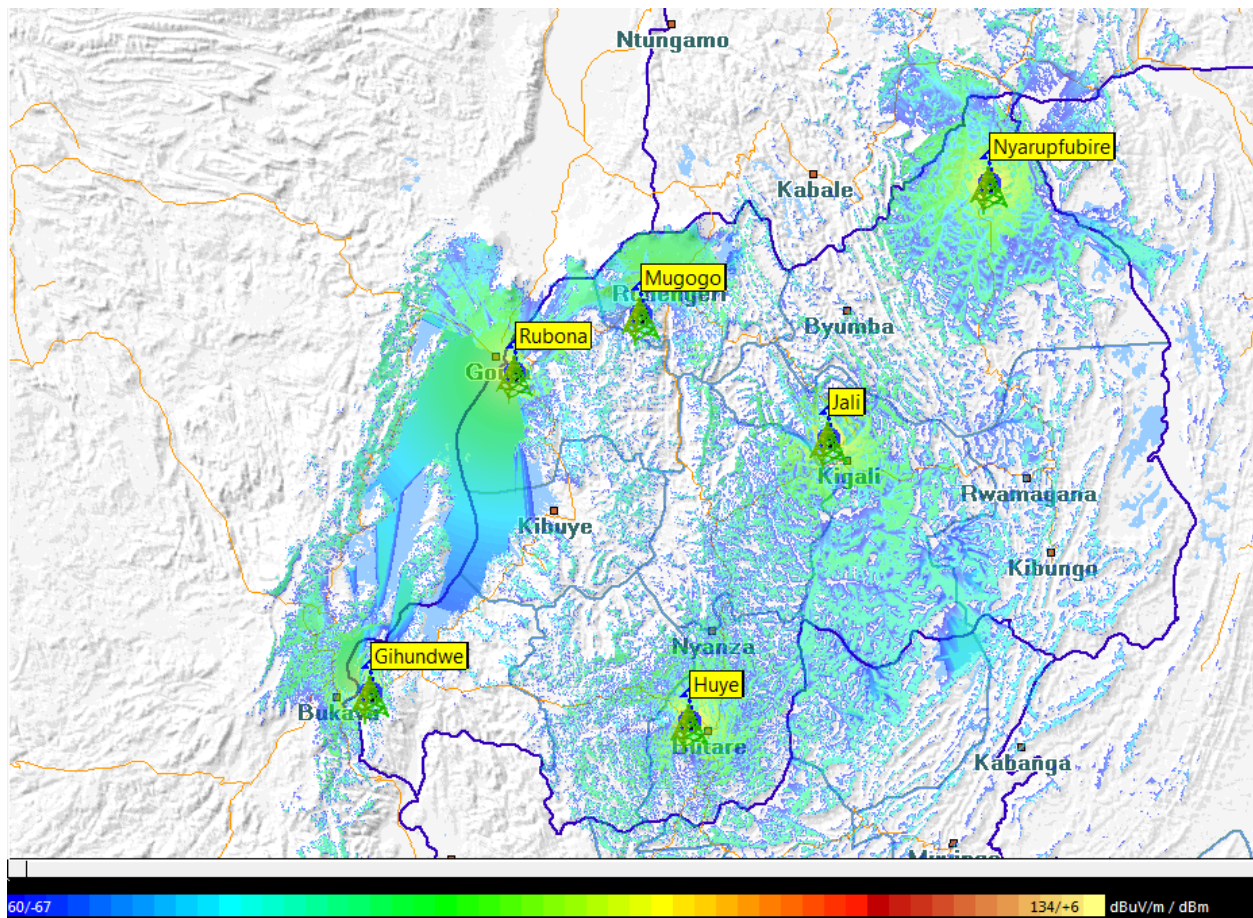
Fig4: PANAFRICA Network Group Ltd Digital TV Network Coverage
