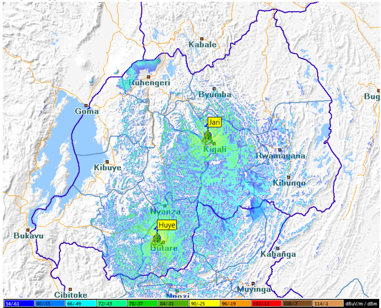
Image 7: Approximate coverage of Salus Radio
