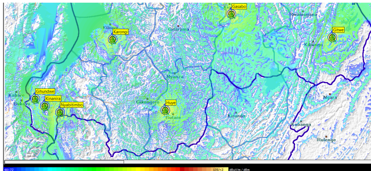
Fig3: Enlarged RBA Digital TV network in the Southern and central part of the country
