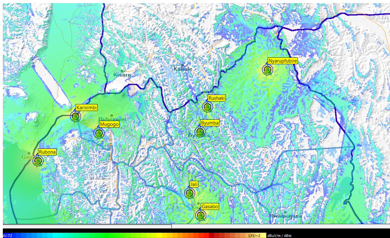
Fig2: The enlarged RBA Digital TV network in the North and Central part of the country
