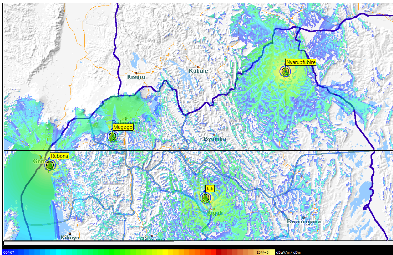
Fig5: Enlarged PANAFRICA Network Group Ltd Network Coverage in the Northern part
