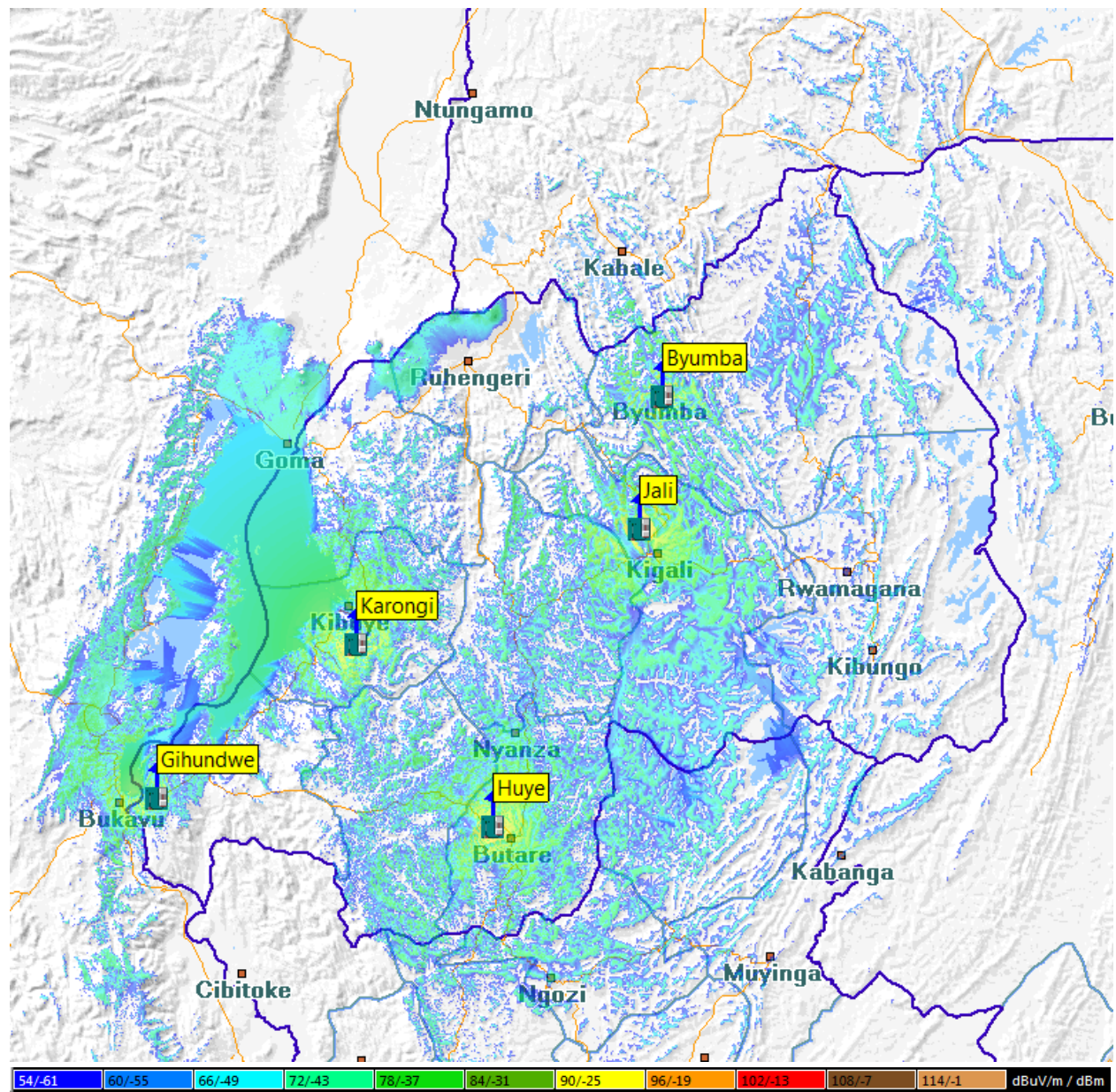
Image 2: Approximate coverage of Radio Maria
