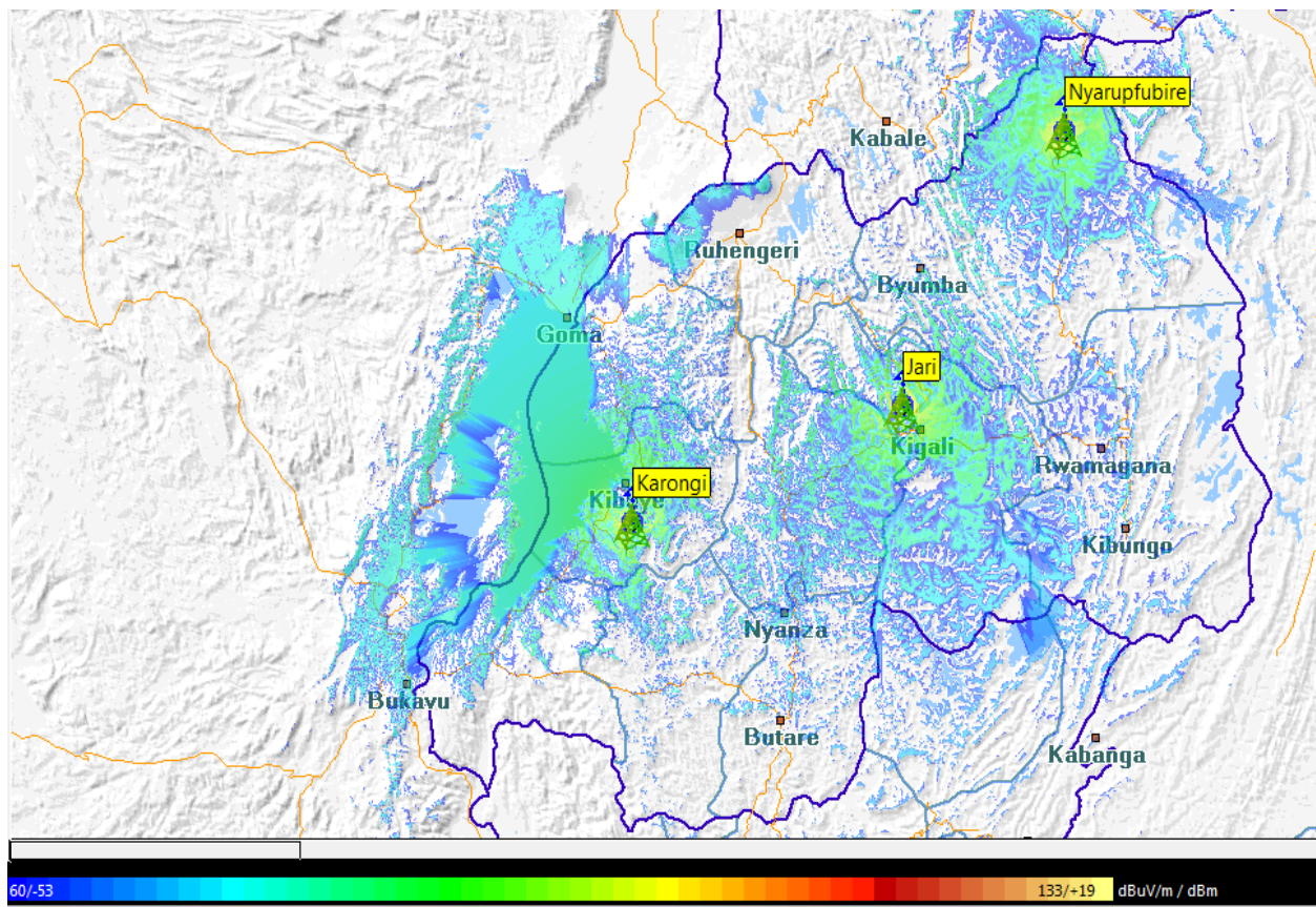
Image6: Approximate coverage of Radio Flash FM
